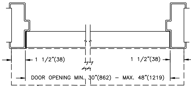
② HORIZONTAL SECTION
