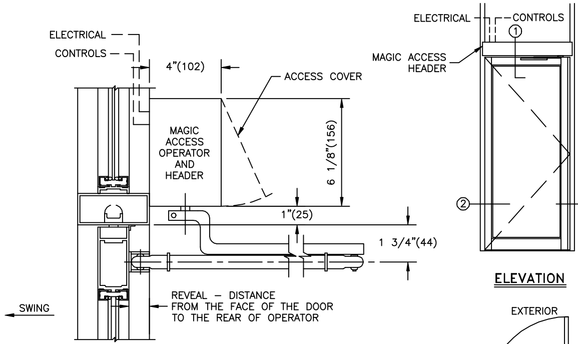
① VERTICAL SECTION
