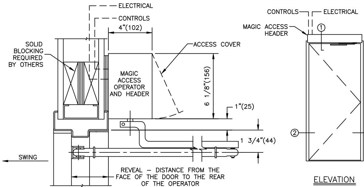
1 VERTICAL SECTION
