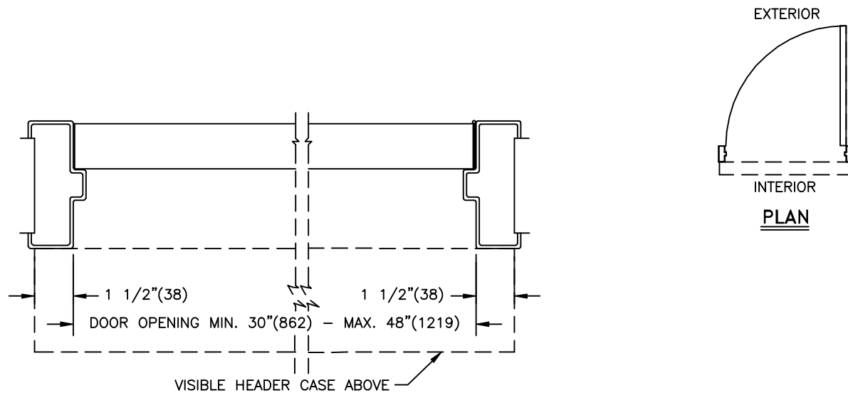
2 HORIZONTAL SECTION
